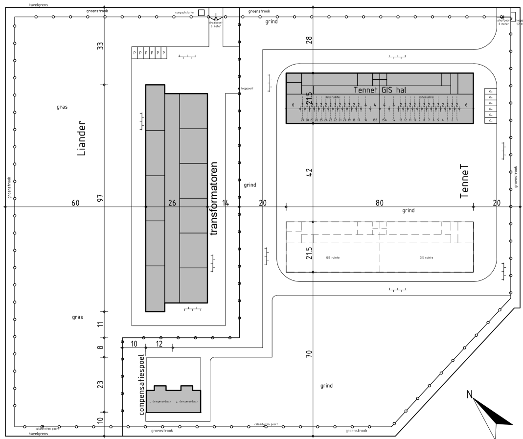
f2.2 Lay-out 150/20 kV-station Incheonweg
