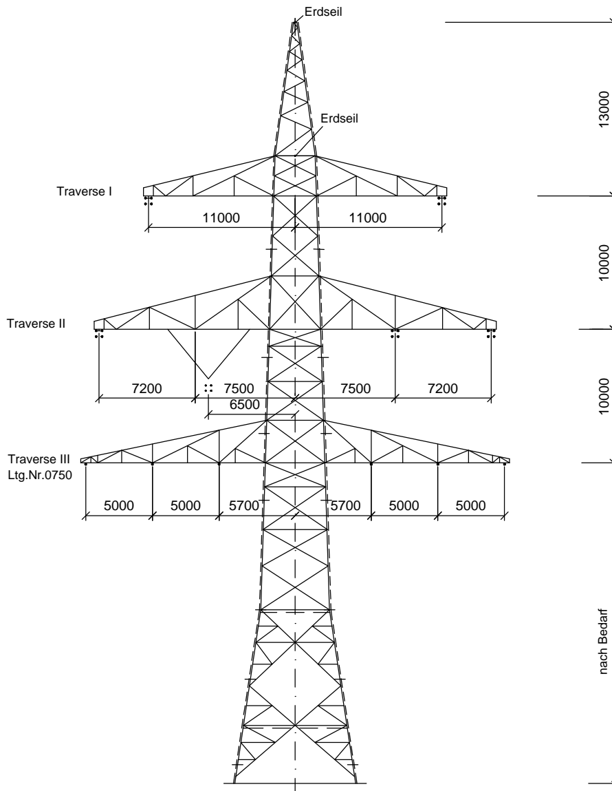
Winkelabspannmast WA120; DA-4-DE-2006.1 Ltg. Nr.309: Mast-Nr. 163 , 178
