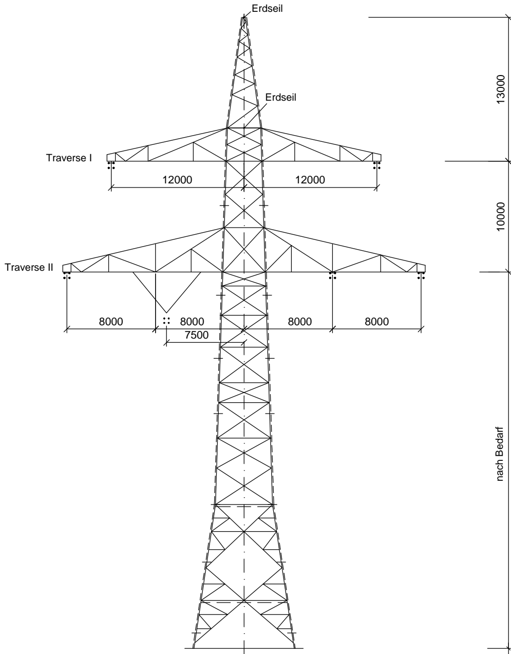
Winkelabspannmast WA100; D-2-D-2006.1 Ltg. Nr.309: Mast-Nr. 12, 125
