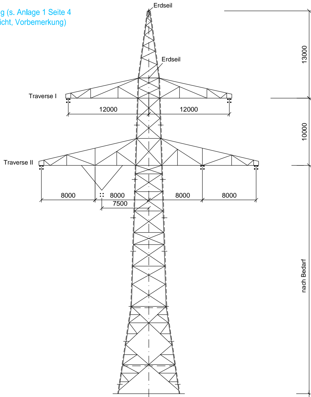
Winkelabspannmast WA100; D-2-D-2009.2 Ltg. Nr.309: Mast-Nr. 12, 111
