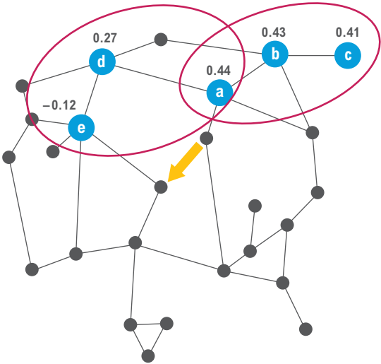
Figure 2.2: An exemplary grid shows five nodes that are to be clustered in zones. The numbers represent PTDFs in respect to the critical line, marked orange. Which alternative would be more desirable from the perspective of market efficiency: a + b + c or a + d + e ?
