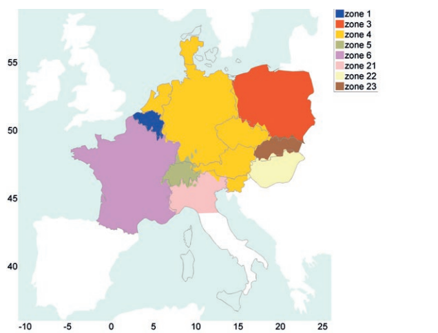
Figure 4.21: Clustering outcome, post adjustment steps 1–4, demonstrating the limitations of the modelling, 2025 SOAF worst case grid (after post-processing steps 1–4)
