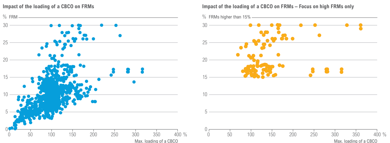
Figure 6.8: Correlation between loading of a CBCO and its FRM
