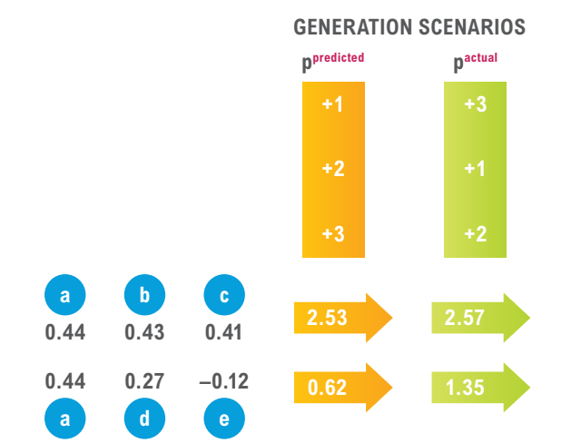
Figure 2.3: If nodes a, b and c inject 1, 2 and 3 units of power respectively, the power flow over the critical branch equals 2.53, whereas shifting the generation pattern to 3, 1, 2 leads to a slightly different result, i.e. 2.57 – the small difference of power flow is caused by the similarity of PTDF values in 'zone' a + b + c .
