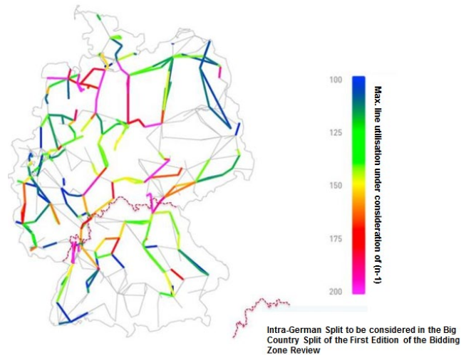
Figure 4.3: Maximum line utilisation under consideration of (N-1) for 2024 (scenario 'Startnetz'); Source: German grid development plan 2014
