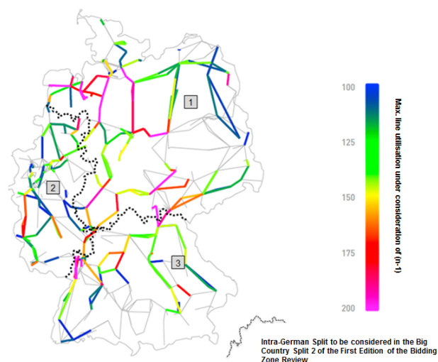
Figure 4.5: Maximum line utilisation under consideration of (N-1) for 2024 (scenario ‘Startnetz’); Source: German grid development plan 2014
