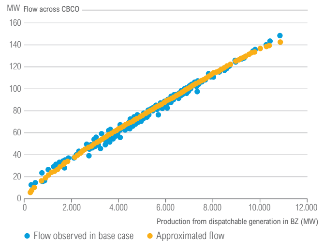
Figure 8.2: Approximation of load flows in the merit-order PTDF approach
