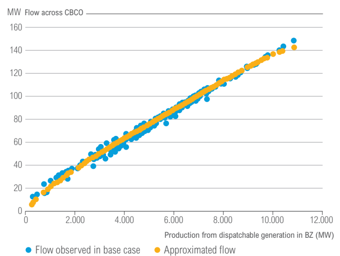
Figure 6.6: Approximation of load flows in the merit-order PTDF approach (for an illustrative line); Note: 'Generation' refers to dispatchable generation only, i.e. excluding variable RES
