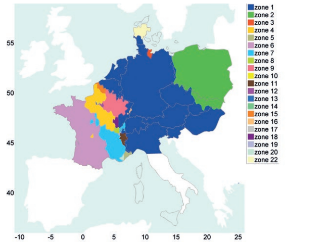
Figure 4.16: Clustering outcome, prior to adjustments, demonstrating the limitations of the modelling, 2025 SOAF planned grid (without post-processing, 22 bidding zones)
