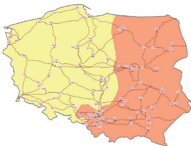
Figure 4.13: PL bidding zone delimitation to be applied in the bidding zone configurations Big Country Split 1 and Big Country Split 2 with the current transmission lines and substations in the background.
