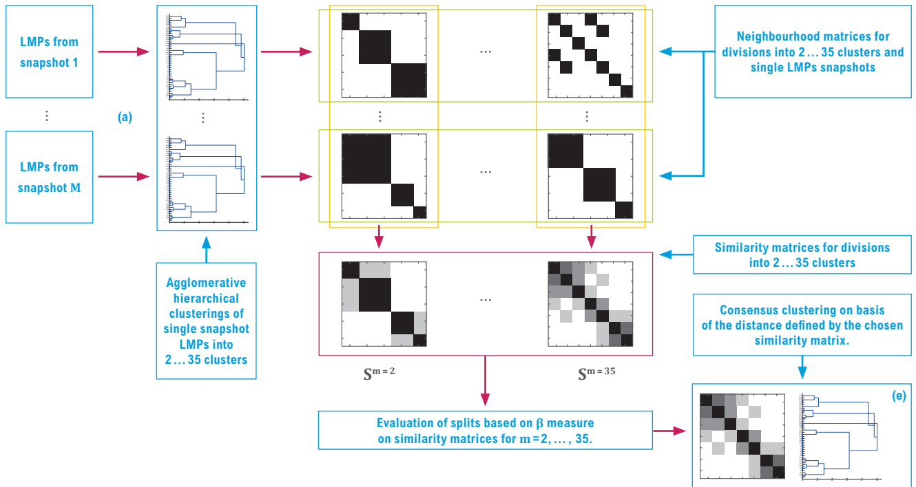
Figure 2.8: Flowchart of the LMP consensus clustering methodology
