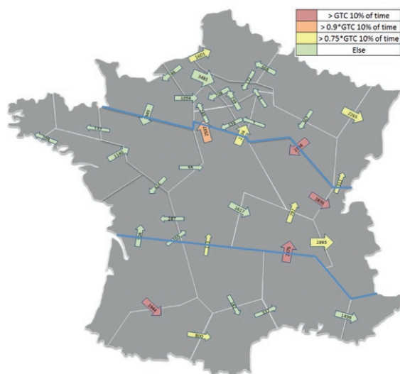
Figure 4.11: Projection with three bidding zones in France
