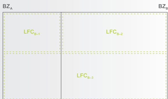
Figure 5.4: One LFC block in several bidding zones (here: in two bidding zones)
