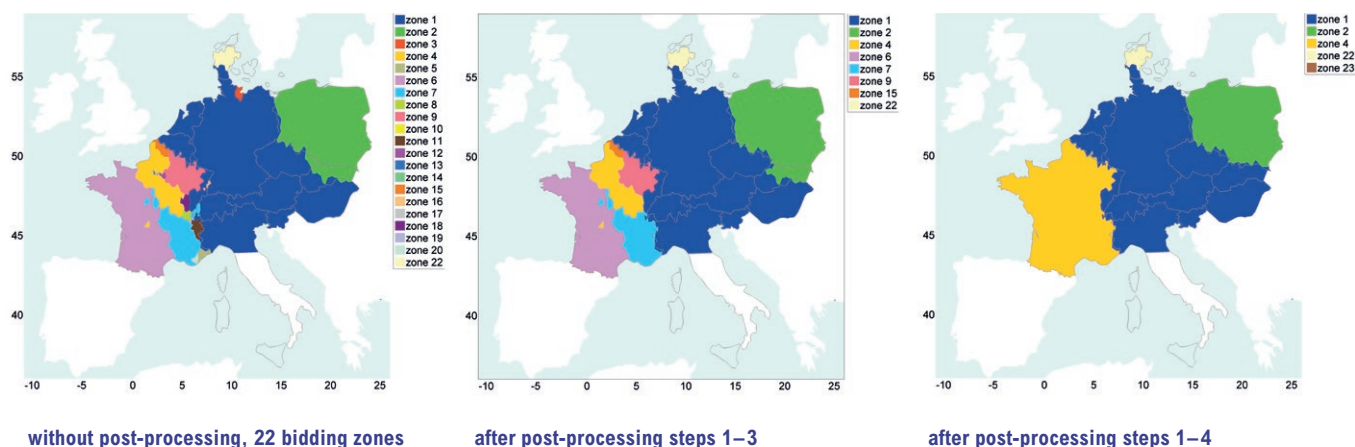
Figure 4.22: Clustering outcome demonstrating the limitations of the modelling, overview of model-based bidding zone configurations; 2025 SOAF planned grid
