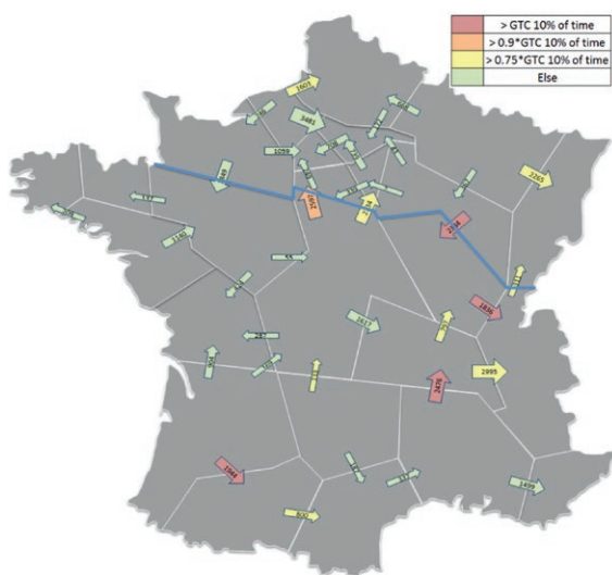
Figure 4.9: Projection with two bidding zones in France
