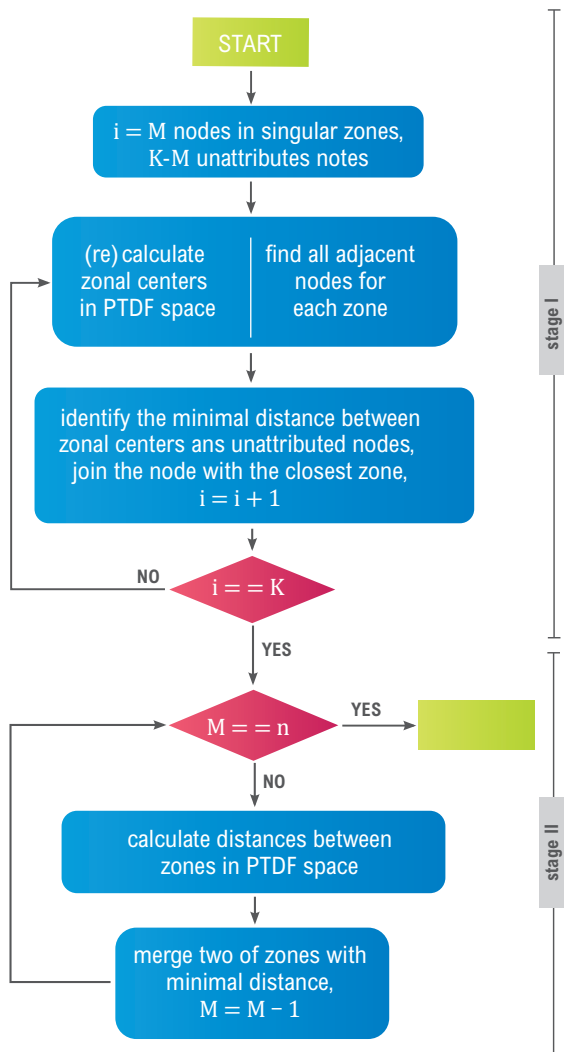
Figure 2.9: Flowchart of the PTDF clustering methodology
