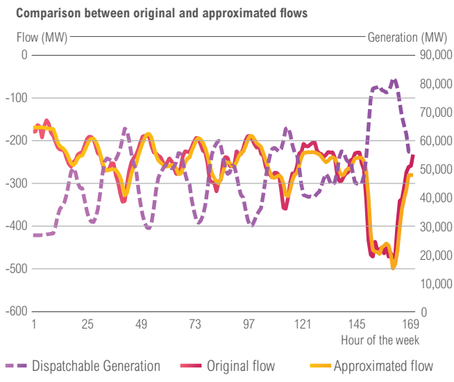
Figure 8.1: Approximation of load flows in the merit-order PTDF approach
