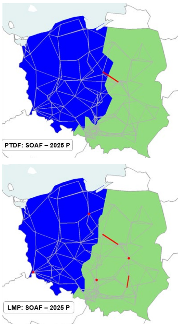
Figure 4.12: PL clustering results by PTDF and LMP methodology for the 'SOAF 2025 grid planned' scenario
