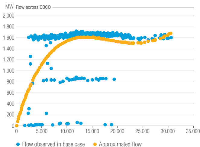
Figure 6.7: Deviations between actual and approximated load flows (for an illustrative line)
