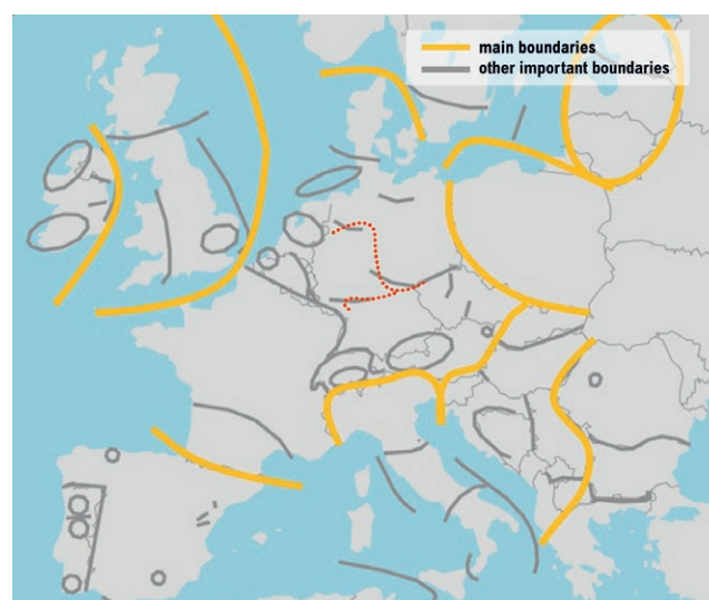
Figure 4.6: Map of the boundaries in Europe including the indicative German bidding zone delimitation applied in the configuration Big Country Split 2 (red dotted line not from TYNDP); Source: Ten-Year Network Development Plan 2016 6)
