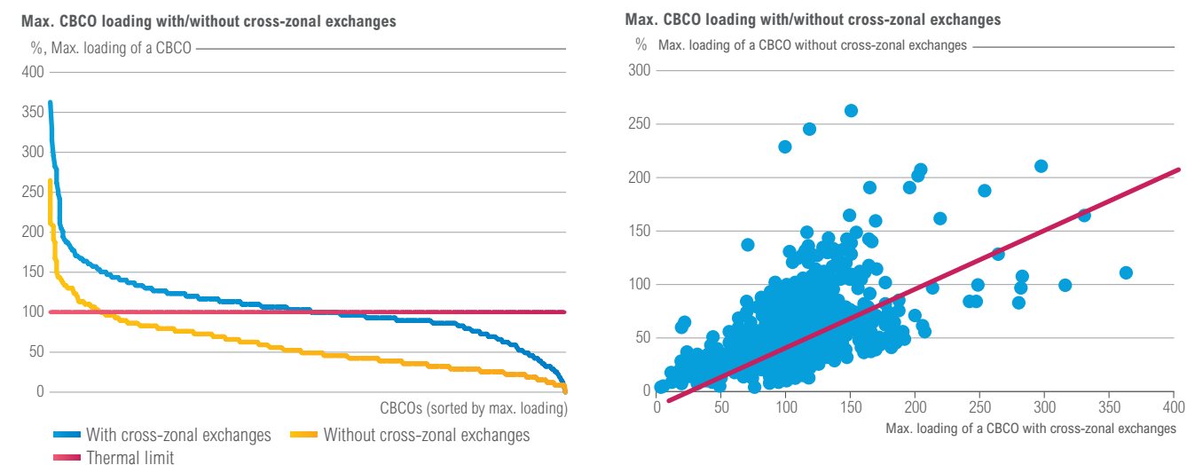
Figure 6.3: Analysis of a pre-congested base case for an illustrative scenario
