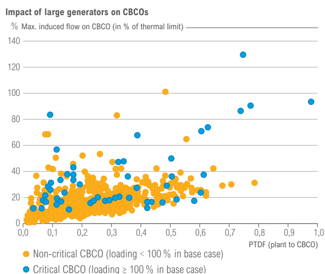
Figure 6.5: Analysis of large plants ( \geq 400 MW) having a significant influence on CBCOs
