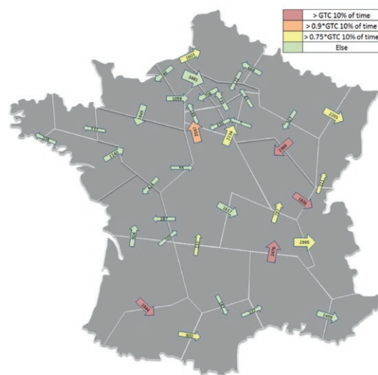
Figure 4.8: Projected physical flows in France in 2030 (MWh/h)
