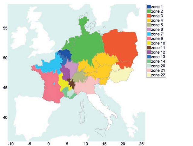
Figure 4.19: Clustering outcome, post adjustment steps 1–3, demonstrating the limitations of the modelling, 2025 SOAF worst case grid (after post-processing steps 1–3)
