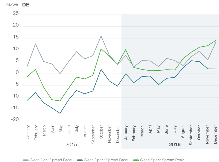
Figure 14: Monthly average clean dark spread base and clean spark spread base/peak in Germany. Calculations based on different assumptions 10 . Source: EPEX Spot, energeate
