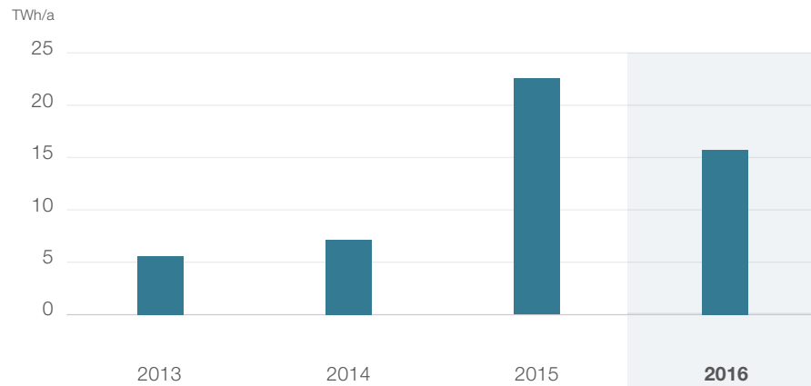
Figure 32: Redispatch volume in Germany from 2013 to 2016 for all requested German TSOs and others with significant volumes 21 . Source: netztransparenz.de
