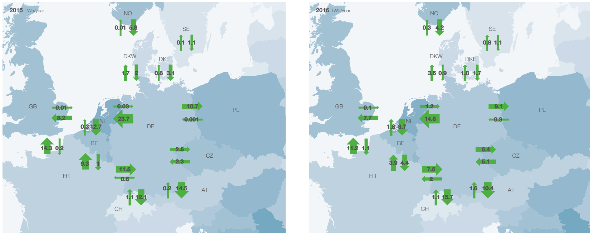
Figure 28: Annual total of physical cross-border flows in the CWE region and at the German borders in TWh. Source: TenneT, ENTSO-E, Swissgrid
