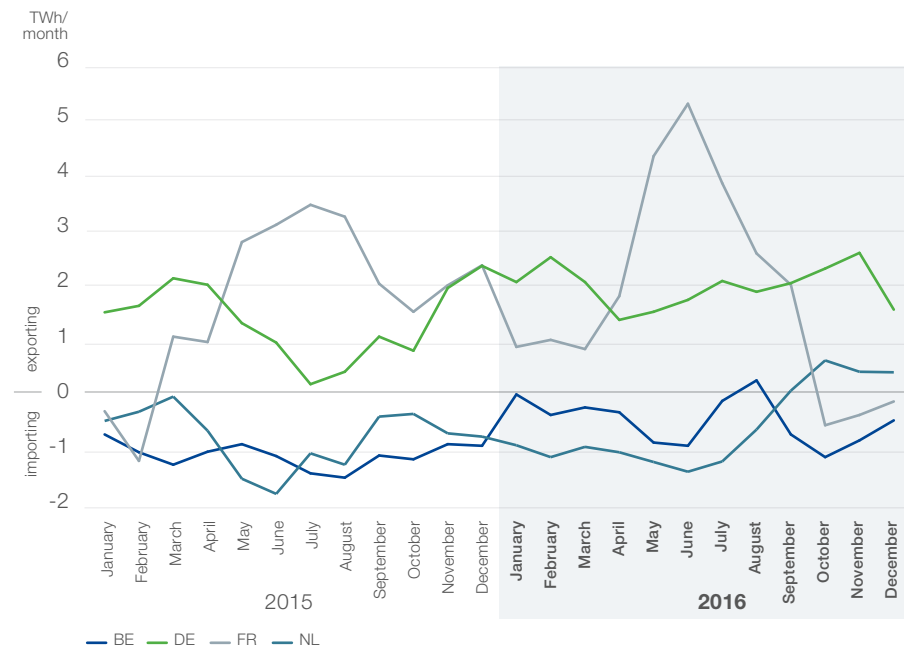
Figure 25: Monthly net positions in CWE countries. Source: ENTSO-E
