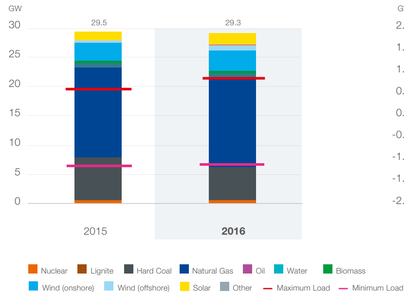
Figure 18: Dutch operational and mothballed generation capacities per fuel type in 2015 (at 1 January 2016) and 2016 (1 January 2017), and the changes in 2016 13 .
