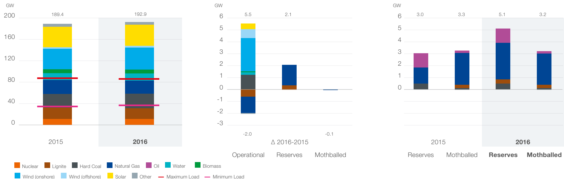
Figure 17: German generation capacities per fuel type in 2015 and 2016. Source: Kraftwerkslisten Bundesnetzagentur, Load: ENTSO-E Generation
