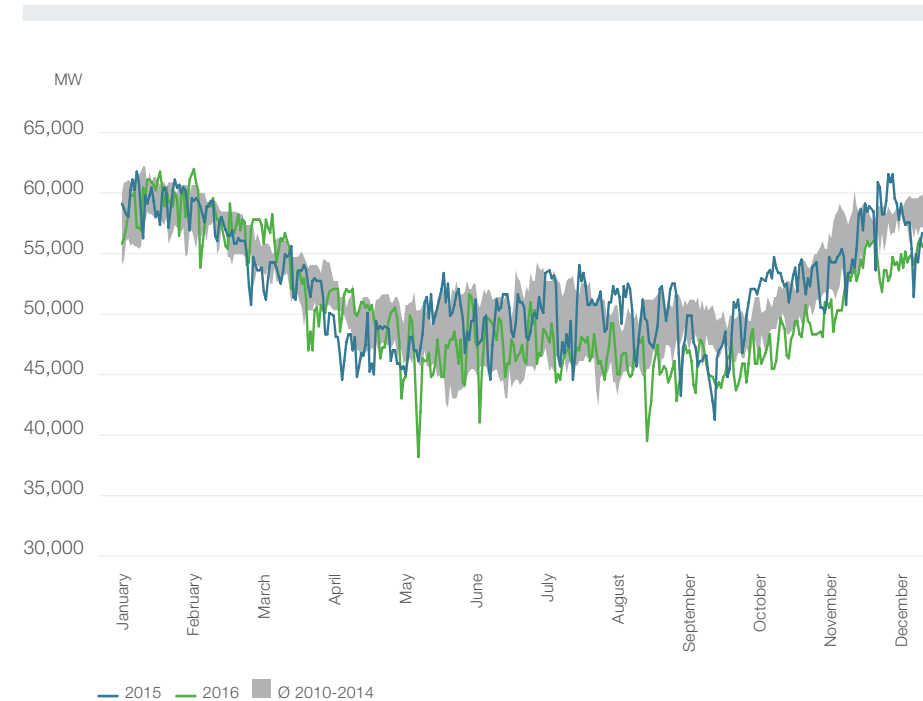
Figure 38: Daily availability of French nuclear power plants. Source: RTE
